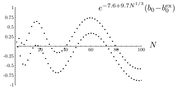
Fig. 5 Oscillations of the strong-coupling coefficient b_0 .
