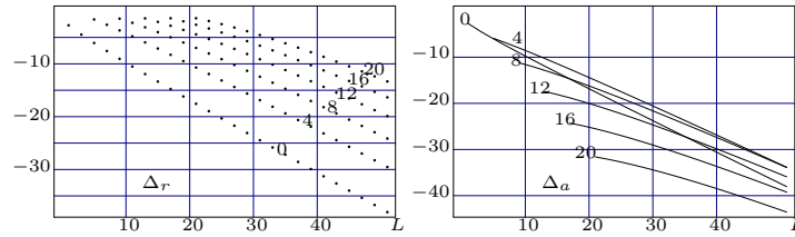
Fig. 18 Relative logarithmic error \Delta_r = \log |1 - b_l^{(L)}/b_l^{(\text{exact})}| on the left, and the absolute logarithmic error \Delta_a = \log |b_l^{(L)} - b_l^{(\text{exact})}| on the right, plotted for some strong-coupling coefficients b_l with l = 0, 4, 8, 12, 16, 20 against the order L .
