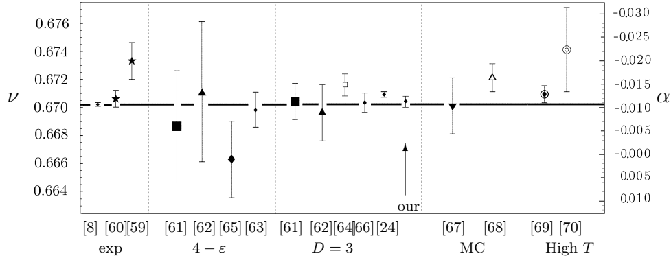
Fig. 9 Survey of experimental and theoretical values for \alpha . The latter come from resummed perturbation expansions of \phi^4 -theory in 4 - \varepsilon dimensions, in three dimensions, and from high-temperature expansions of XY-models on a lattice. The sources are indicated below.
